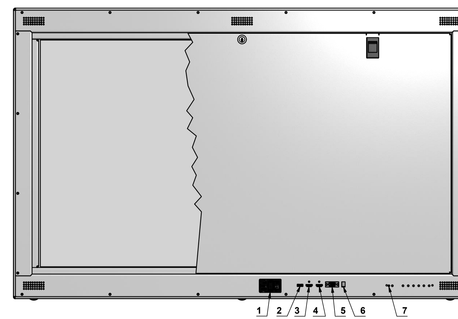
Back View 1:5
