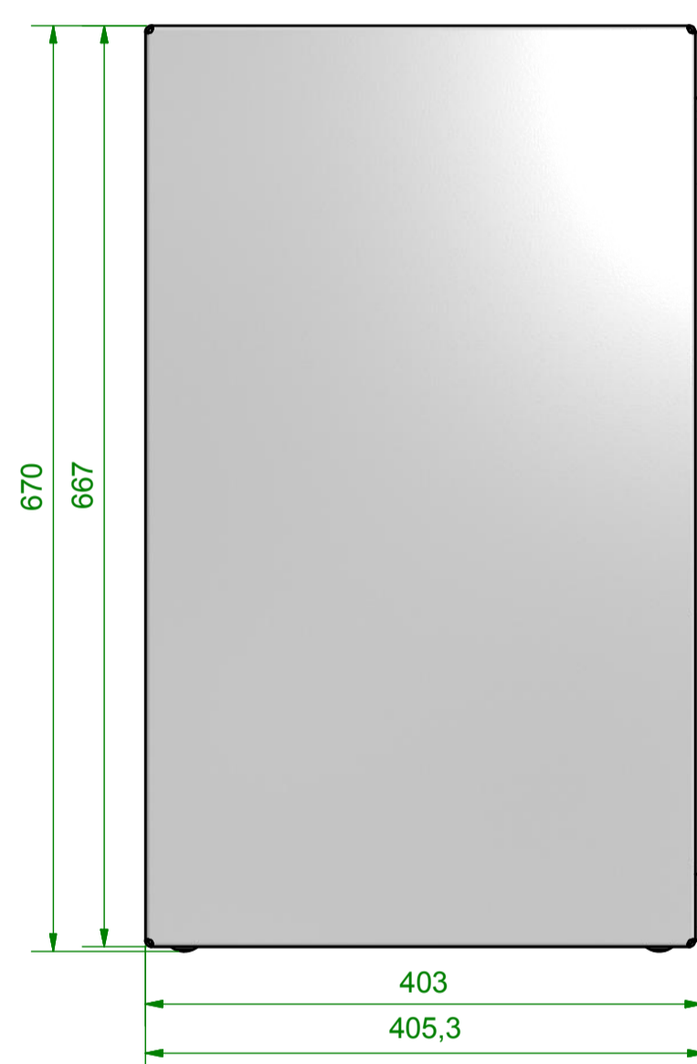
Righthand View 1:5
