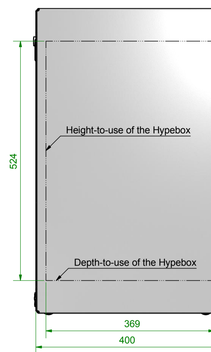
Lefthand View 1:5
