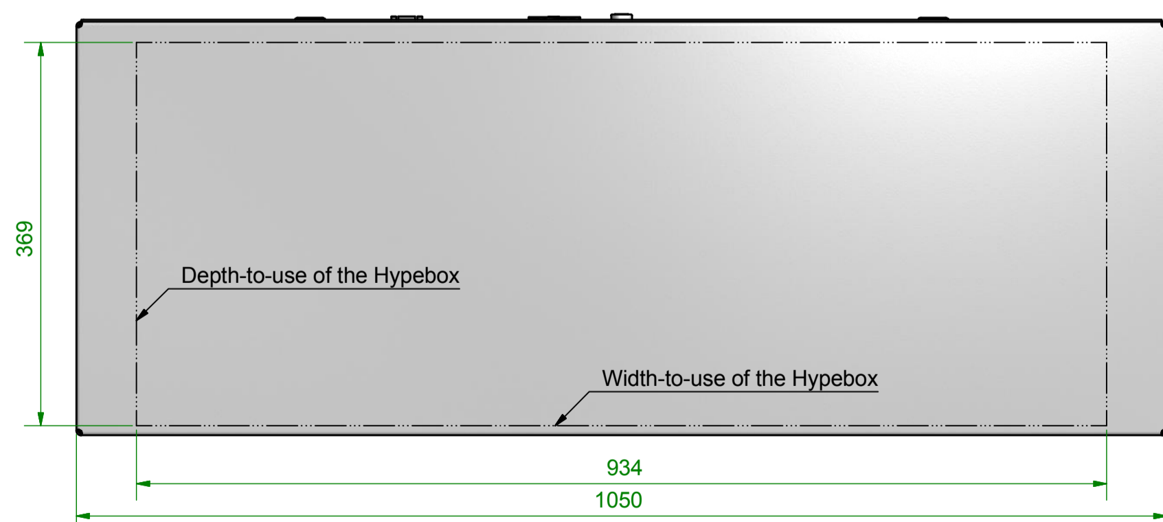
Top View 1:5
