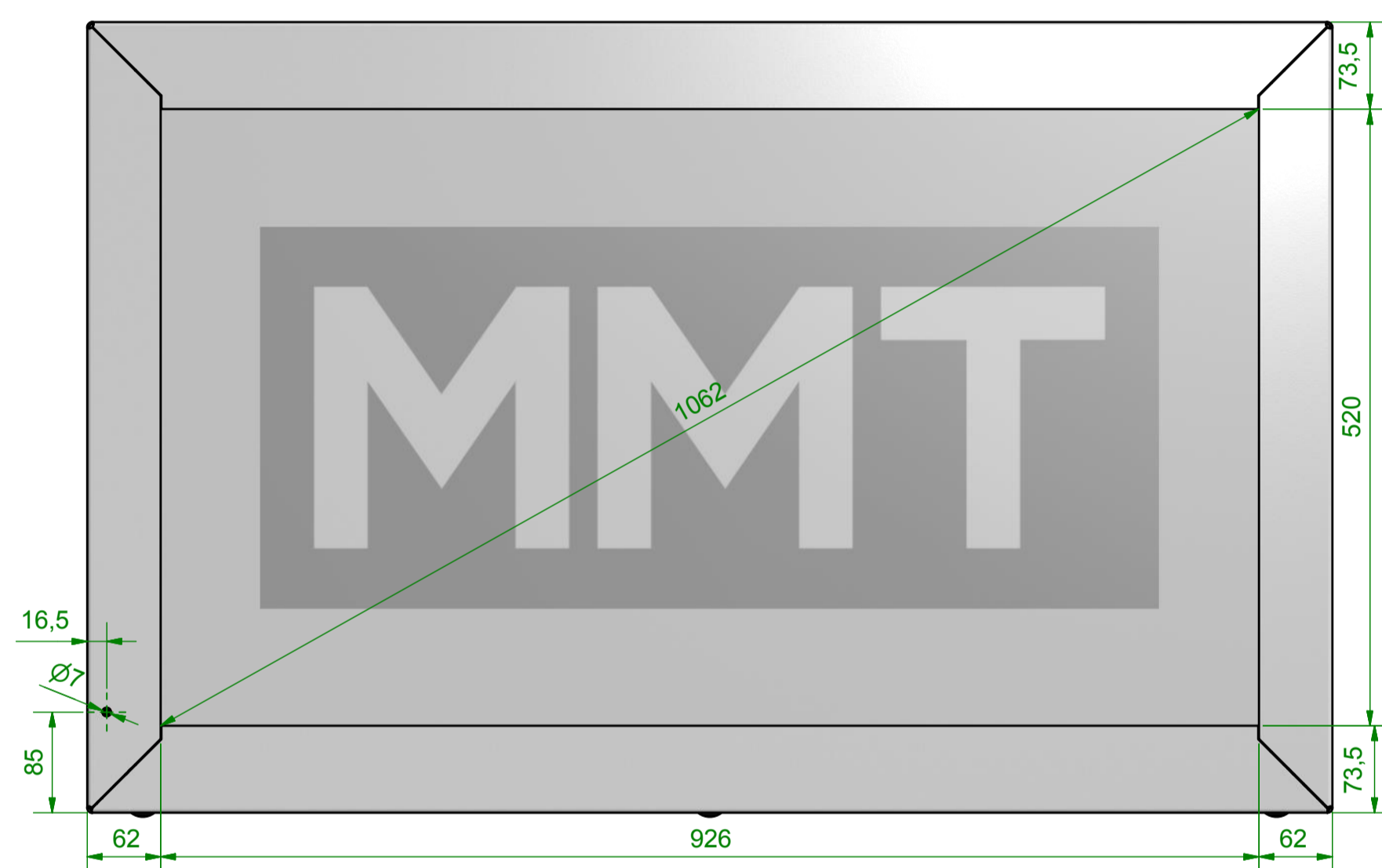
Front View 1:5
