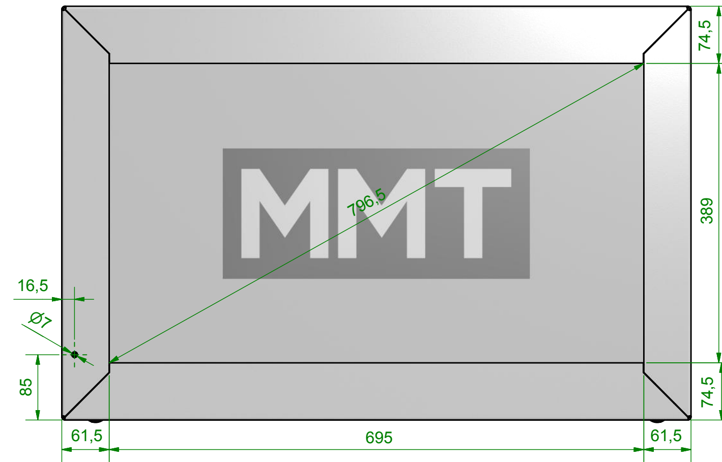
Front View 1:5
