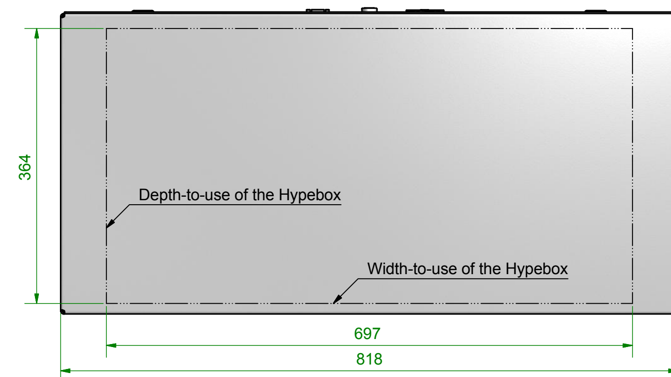
Top View 1:5
