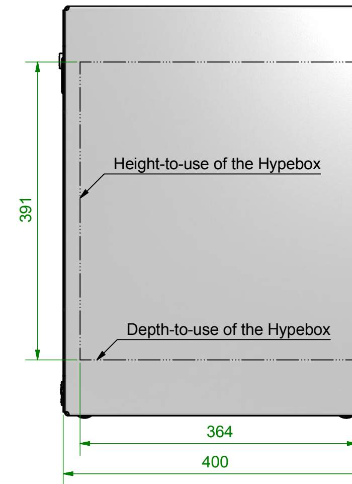
Lefthand View 1:5
