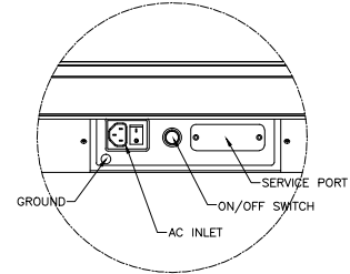
VIEW "A" SCALE 2:1
