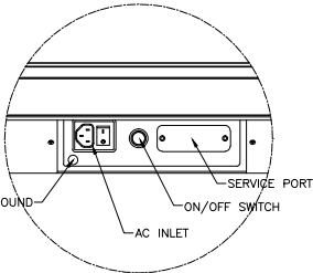
VIEW "A" SCALE 2:1
